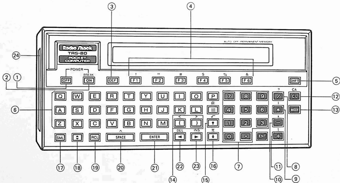
Figure 1. PC-2 (Front View)
